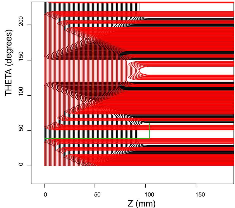
SCQ Serpentine: Close Up at Lead End
