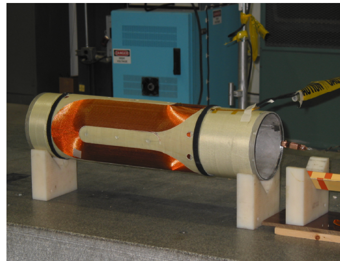
Warm coil testing before vacuum impregnation was done and the fiberglass prestress wrap was added.
