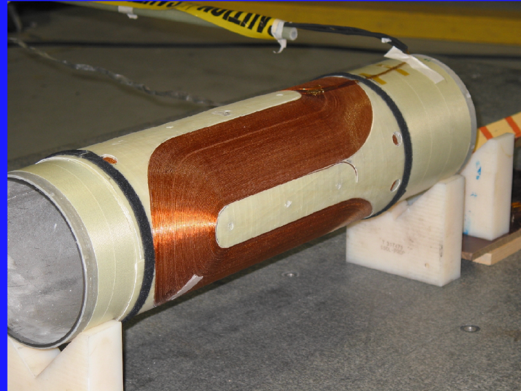
Serpentine Test Winding
