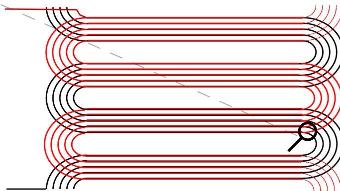
Double-Layer Winding Schematic.
