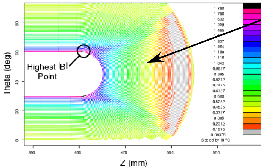
|B| per ampere of excitation current for wire segments in lower coil layer.
